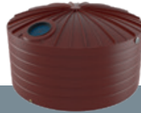
10000L (2200gal) TXD2200 SQUAT Inlet (H) 1.55m (5'1") Diameter 3.08m (10'1") Total (H) 1.81m (5'11")
